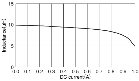
VLS252015T-100MR66
